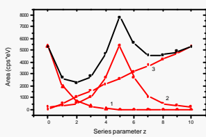
Fig. 5. Calculated areas in dependence on series parameter z: Black curve: total area after background subtraction only. Red curves (1-3): single peak areas 1-3 after batch processing with UNIFIT 2001
